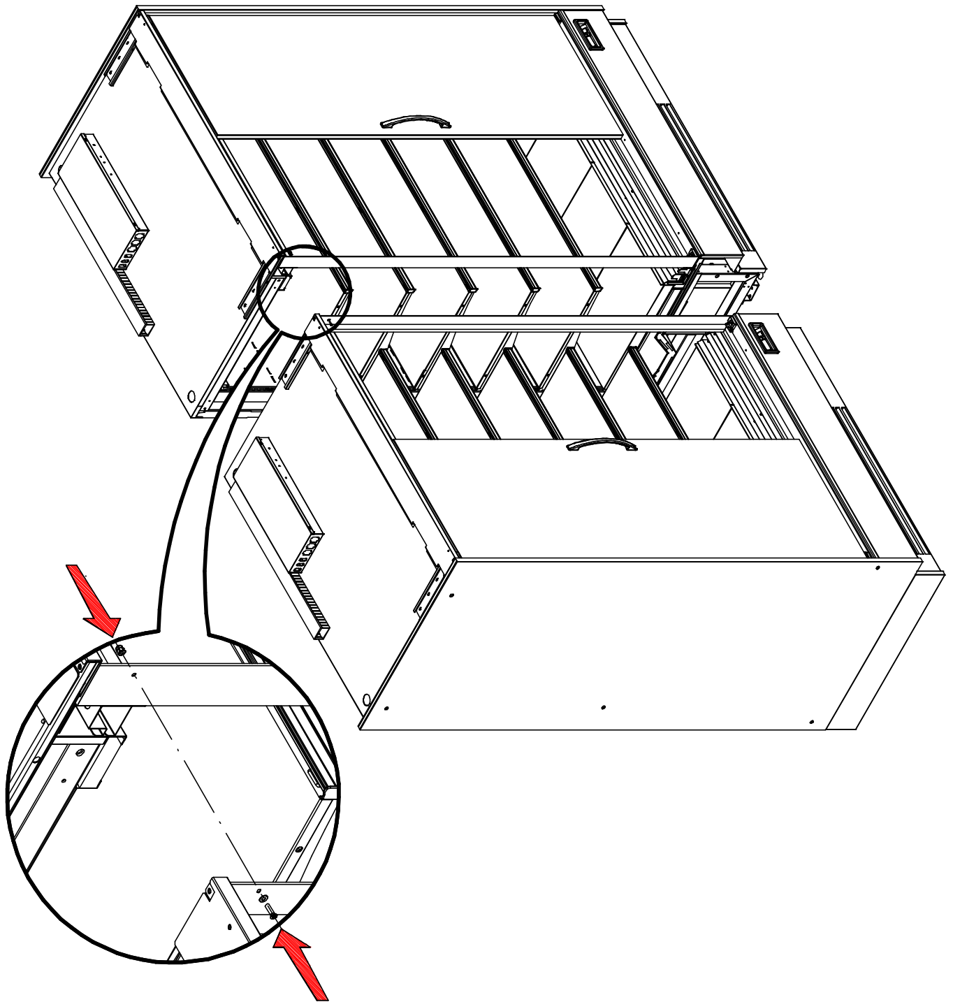
FIG. 18 VISION DOORS
