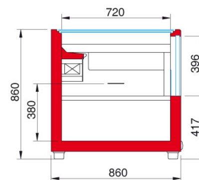
Header model
