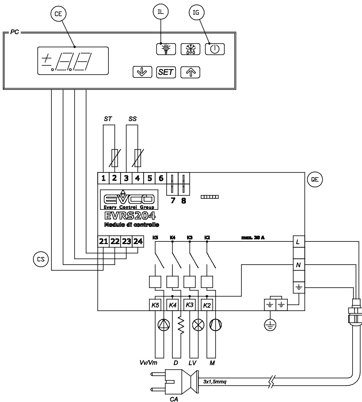
FIG. 32 - VERSIONI REFRIGERATE / REFRIGERATED VERSIONS
